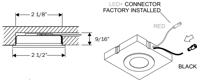
511 050 Recessed Mount
